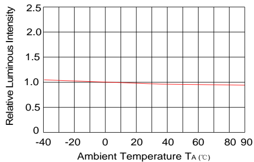
Fig.4 Relative Intensity Vs. Ambient Temperature
